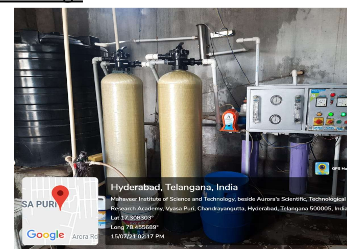
RO System
